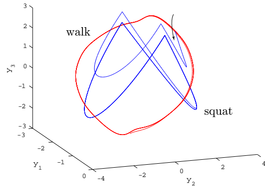
Figure 9: Transition of motion from “walk” to “squat” ( \varepsilon_{ws} = 500 ).
