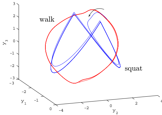
Figure 8: Transition of motion from “walk” to “squat” ( \varepsilon_{ws} = 5 ).
