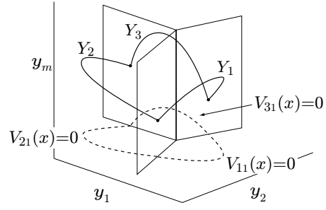
Figure 6: Piecewise quadratic Lyapunov function V_{q_1} .
