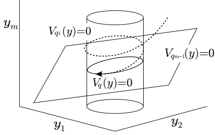
Figure 5: An ellipsoidal curve defined by an elliptic cylinder and a hyperplane.
